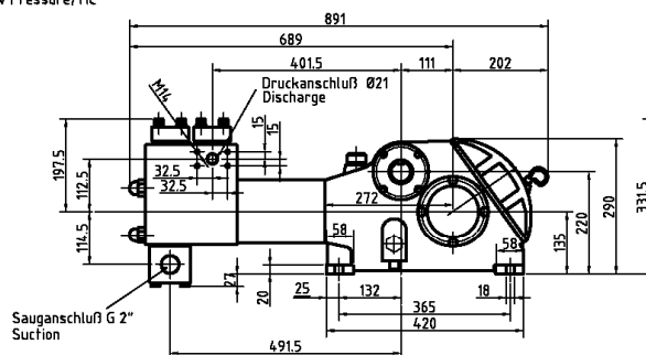
Niederdruckkopf MC Compact Head (Low Pressure) MC
