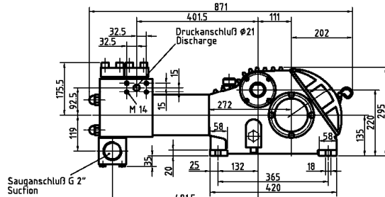
Niederdruckkopf MC Compact Head (Low Pressure) MC
